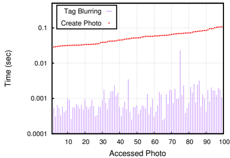
Figure 11: The total time required for serving a photo, which includes reading the access permission and blurring a face.
