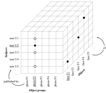
Figure 7: Visualization of our revised access control model.
